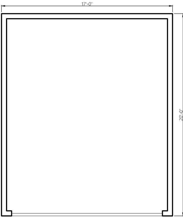
(E) Floor Plan ( Garage)
